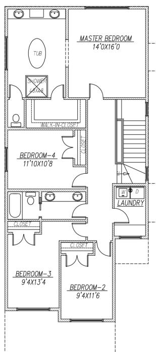
UPPER FLOOR PLAN (4 BEDROOM) 1287 SQ FT
