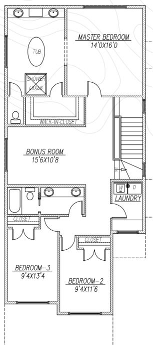
UPPER FLOOR PLAN 1287 SQ FT
