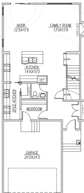
MAIN FLOOR PLAN (SPICE KITCHEN) 1056 SQ FT
