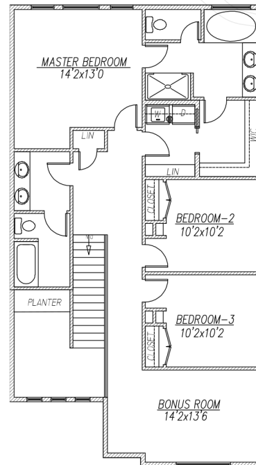
UPPER FLOOR PLAN (OPEN ENTRY) 1197 SQ FT
