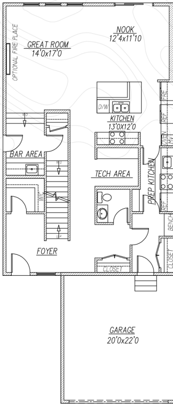
MAIN FLOOR PLAN (PREP KITCHEN) 1225 SQ FT
