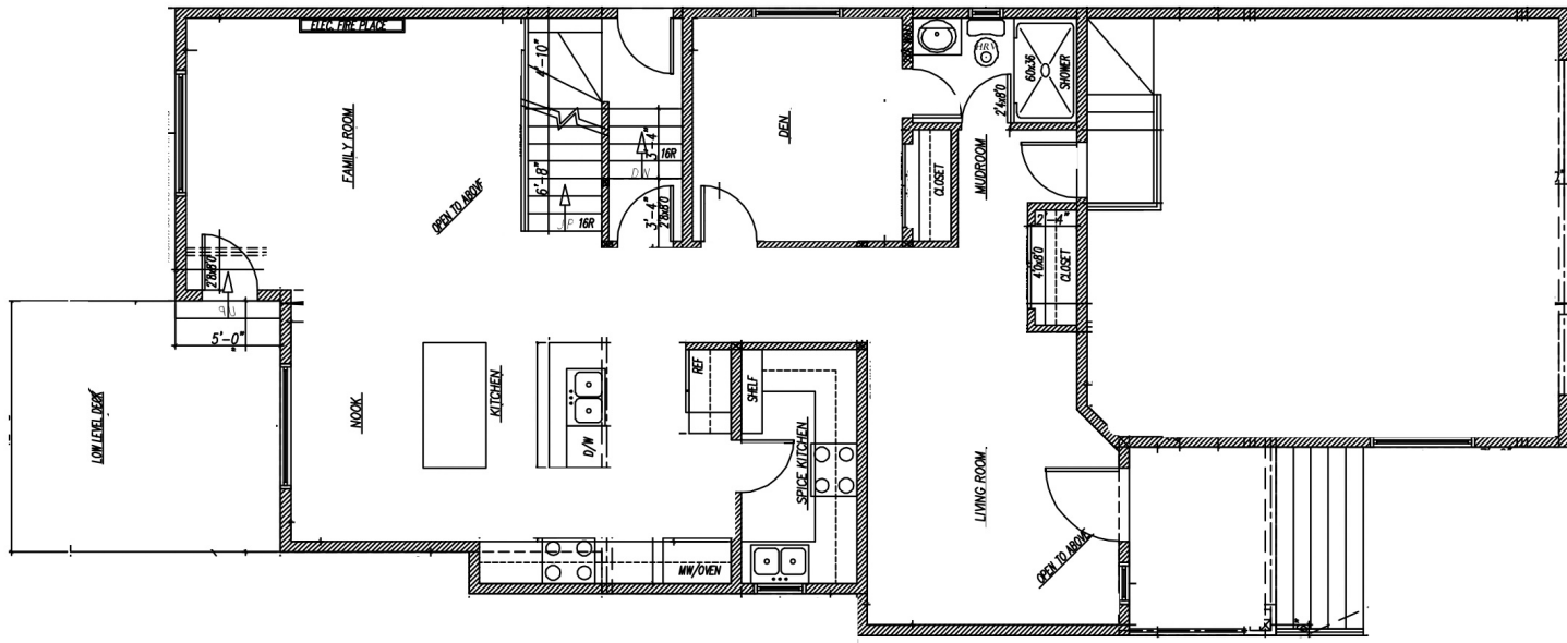
MAIN FLOOR PLAN 1172 SQ.FT. GARAGE 492 SQ.FT.
