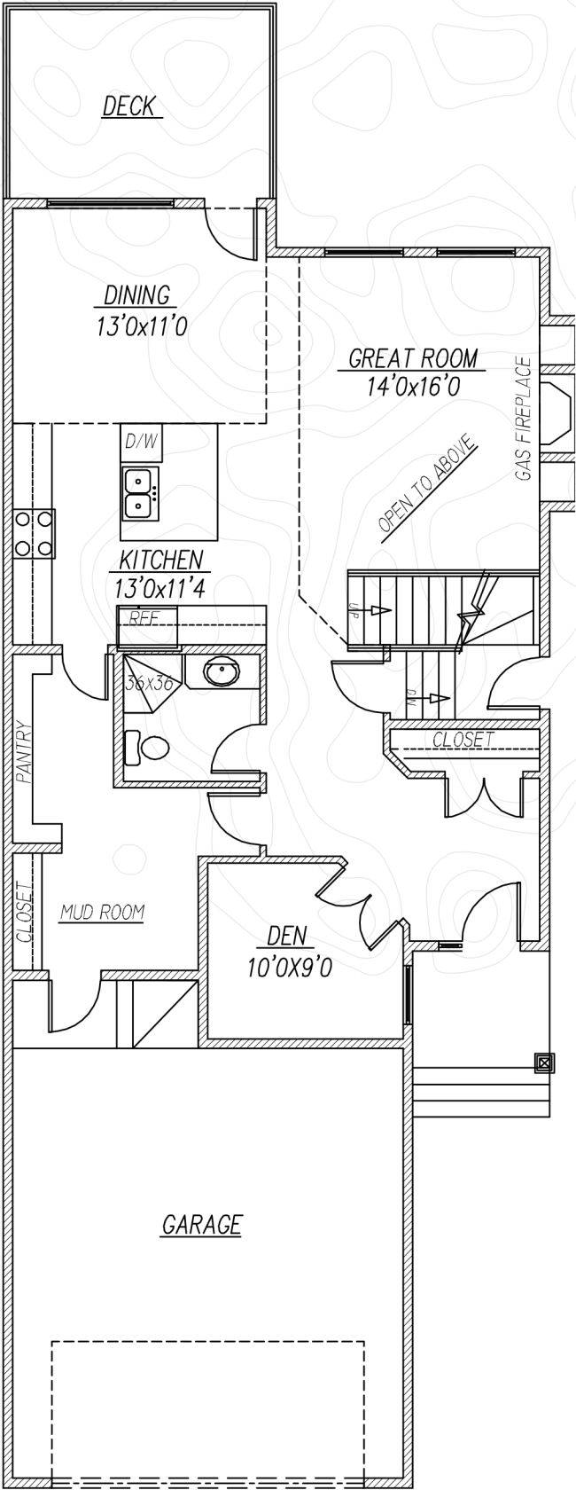
MAIN FLOOR PLAN 1131 SQ FT
