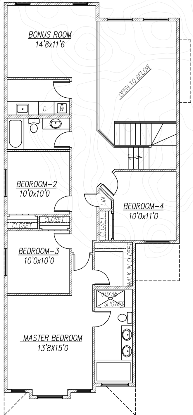
UPPER FLOOR PLAN (4 BEDROOMS) 1258 SQ FT
