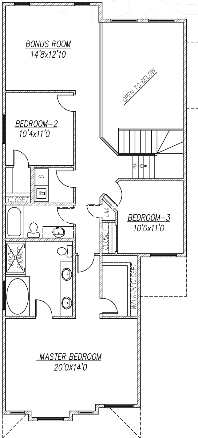
UPPER FLOOR PLAN 1258 SQ FT
