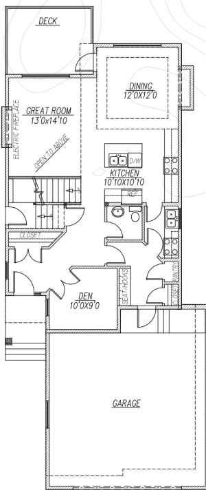
MAIN FLOOR PLAN (SPICE KITCHEN) 996 SQ FT
