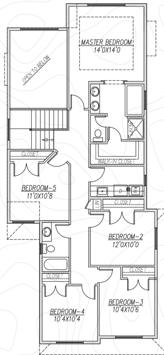
UPPER FLOOR PLAN (5 BEDROOM) 1263 SQ FT
