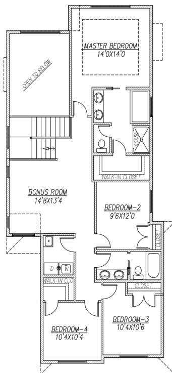
UPPER FLOOR PLAN (ALTERNATE UPPER) 1263 SQ FT
