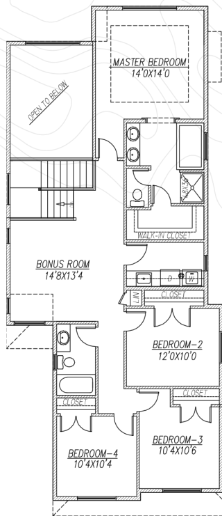
UPPER FLOOR PLAN 1263 SQ FT
