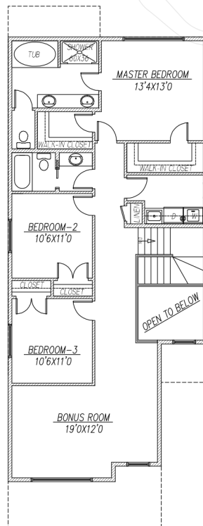
UPPER FLOOR PLAN (OPEN ENTRY) 1251 SQ FT
