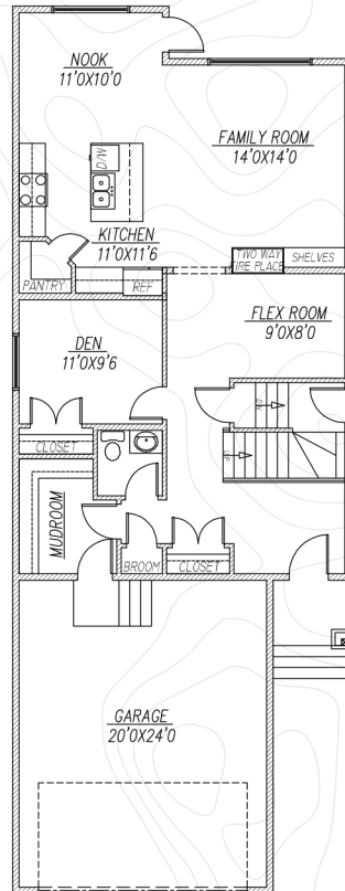
MAIN FLOOR PLAN (DOUBLE SIDED FIREPLACE) 1088 SQ FT
