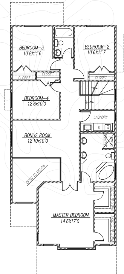
UPPER FLOOR PLAN (BONUS ROOM WITH 4 BEDROOMS) 1370 SQ FT
