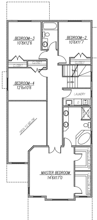
UPPER FLOOR PLAN 1260 SQ FT
