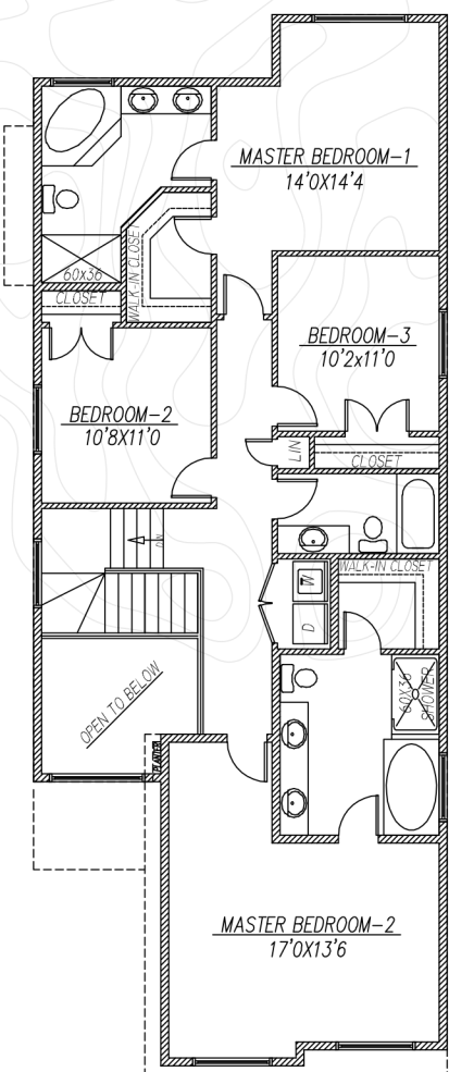
UPPER FLOOR PLAN (DUAL MASTERS WITH 2 BEDROOMS) 1342 SQ FT
