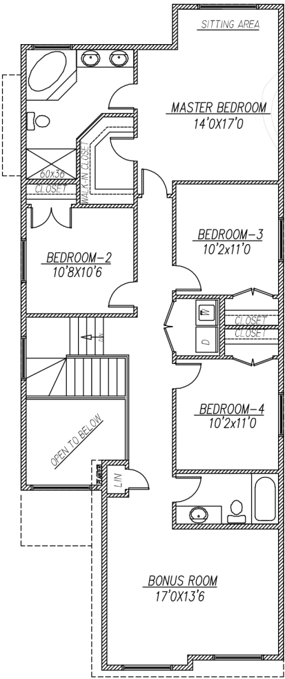
UPPER FLOOR PLAN 1343 SQ FT
