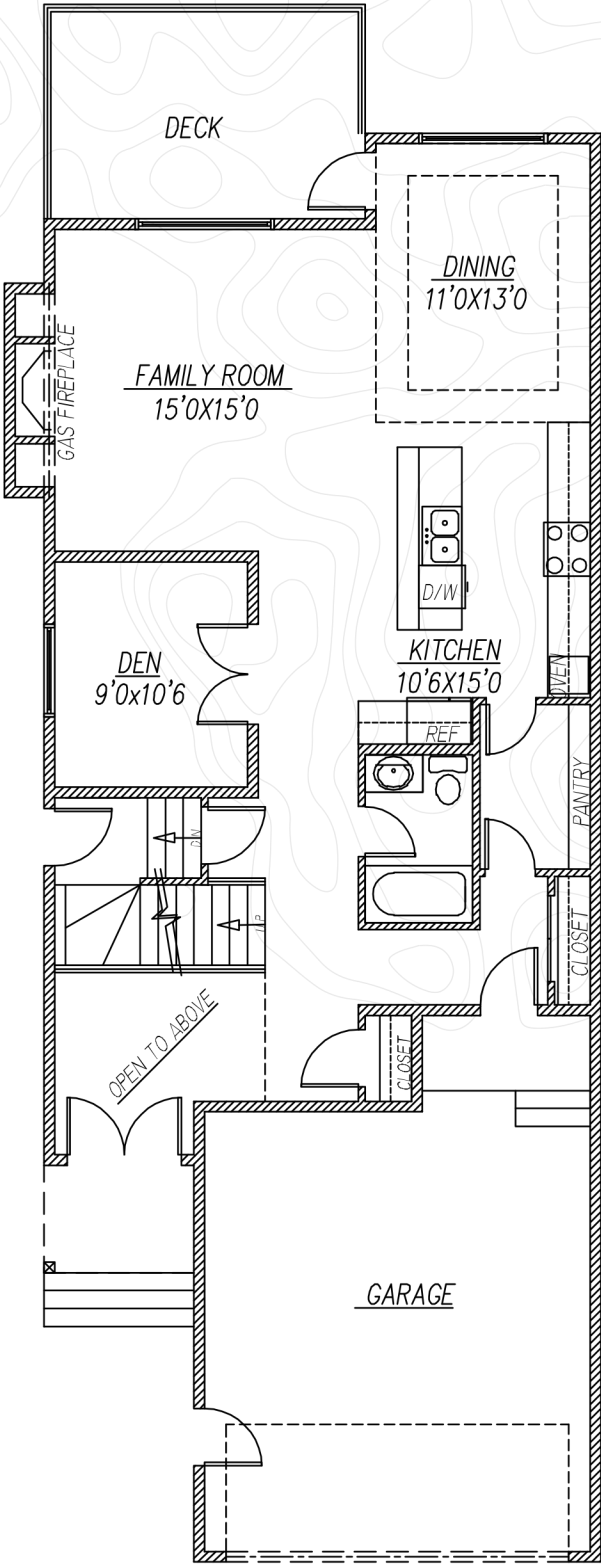
MAIN FLOOR PLAN 1127 SQ FT
